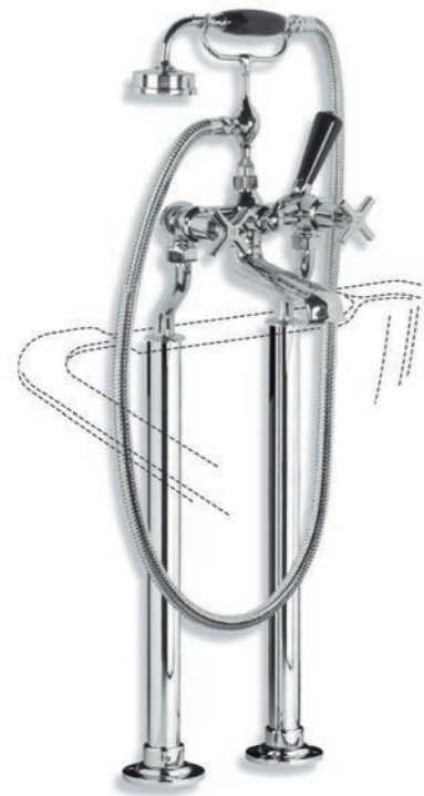
MH 1145 MACKINTOSH BATH SHOWER MIXER WITH STANDPIPE SLEEVES & ADJUSTABLE BASEPLATES FOR RIM MOUNTING
